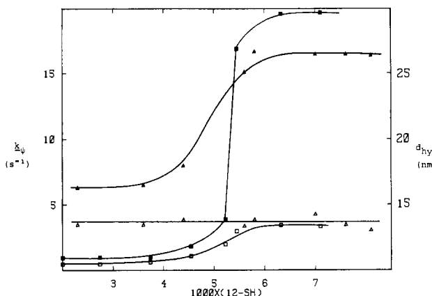
Figure 2. (a) k_{\psi} (s -1 ) (left-hand ordinate) vs. 10 3 [12-SH] (M) for the cleavages of LL-2 (■) or DL-2 (□) by micellar 12-SH; cf. Table II. For clarity, k_{\psi}^{LL} has been arbitrarily increased by 0.5 s -1 at each point. (b) Apparent hydrodynamic diameters (nm) (right-hand ordinate) of 12-SH micelles vs. 10 3 [12-SH] (M) after reactions at pH 8 with 2.0 \times 10^{-5} M LL-2 (▲) or DL-2 (△); cf. Table V, run 1.
